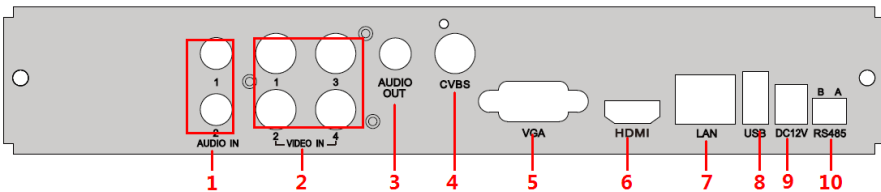
Fig 2-3 Rear Panel for 4-ch
