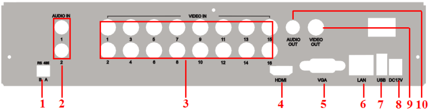
Fig 2-5 Rear Panel for 16-ch
